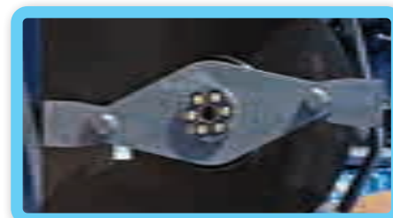
Two double-sided blades on a 5/8" thick blade carrier
