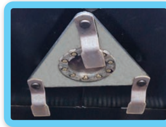
60" unit features three double-sided blades on a 3/4" thick blade carrier
