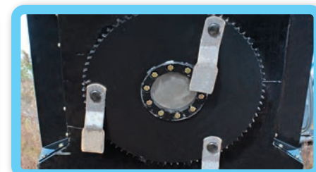
Three dropdown blades on a 1" thick blade carrier
