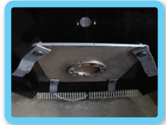
72" unit features four double-sided blades on a 3/4" thick blade carrier
