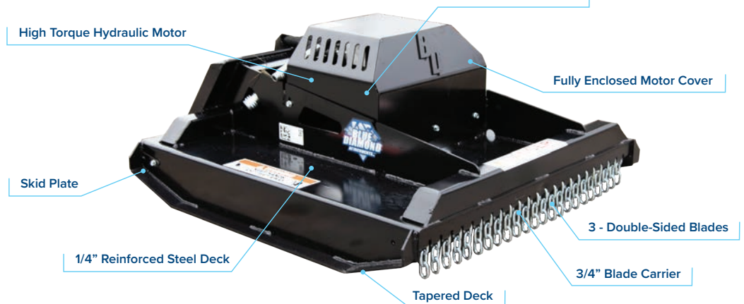
Three double-sided blades on a 3/4" thick blade carrier
