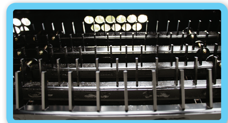
Replaceable and reverseable rake bars w/AR400 hardened steel teeth
