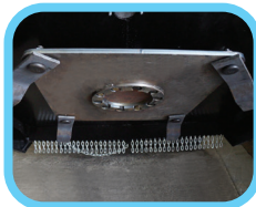
72" unit features four double-sided blades on a 3/4" blade carrier
