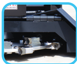
1" thick hinged deflector
