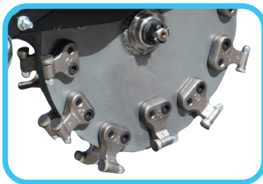
Dual direction cutting with teeth on both sides of wheel
