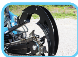
Self-adjusting crumber sweeps the trench clean
