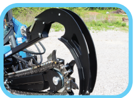
Spring-loaded self-adjusting crumber sweeps the trench clean
